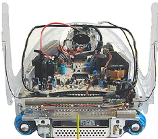
Divider Panel
