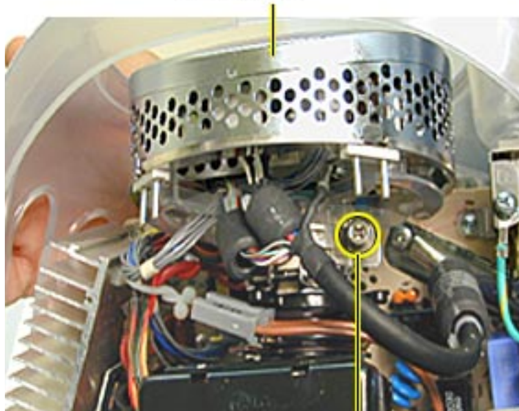
CRT Neck Screw
