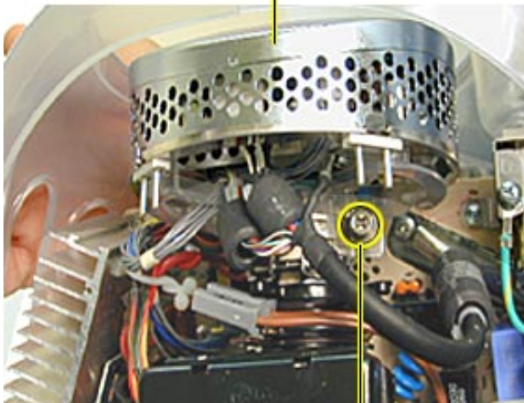
CRT Neck Screw
